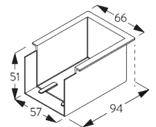
SG 11885 Recess mask
