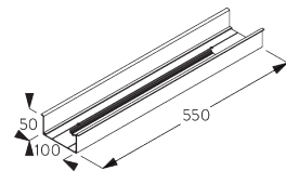
SG 11846 Recess box right
