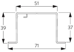
SG 2932 Recess profile
