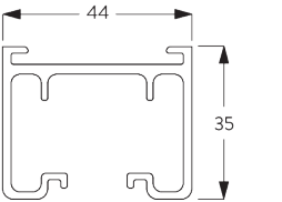
SG 2901 Profile
