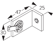
SG 3181 Bracket 1 clamp
