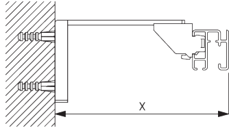
Smart Fix SG 11200 - SG 11205 and bracket SG 3603: Screw SG 10492 (M4x8) needed.
